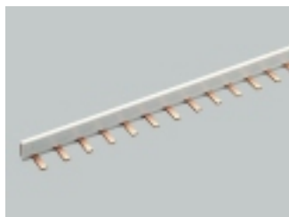
31101 comb type busbar, insulated, 1-pole, bridge type 75 A, pitch 27 mm, 1 m long
